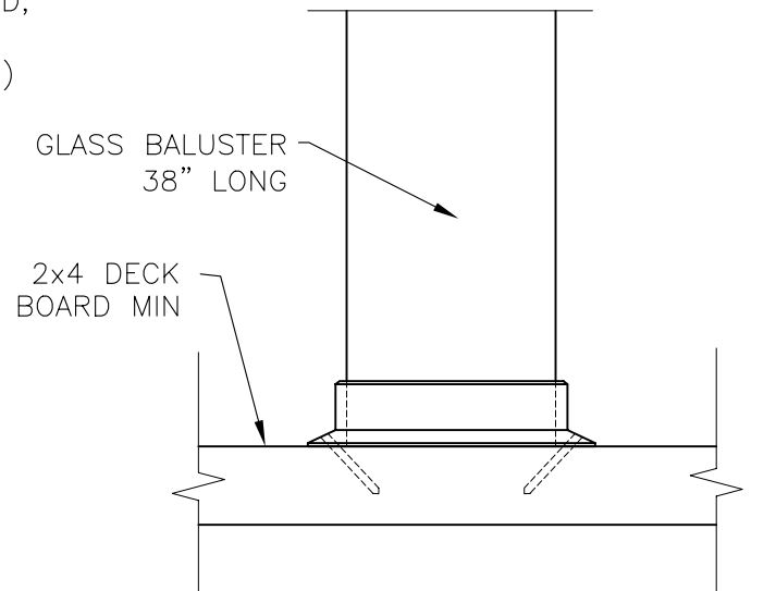
T S9 ALT GLASS BALUSTER CONNECTION
