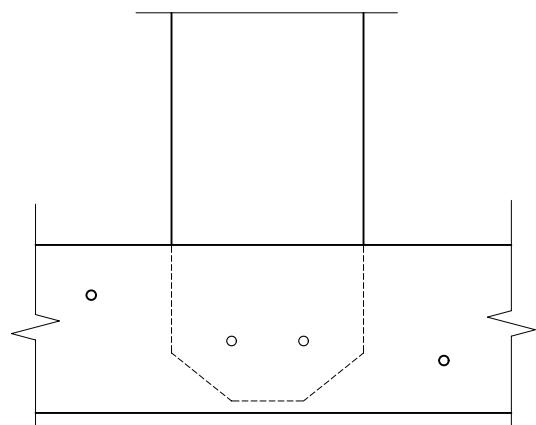
L S9 GLASS BALUSTER CONNECTION
